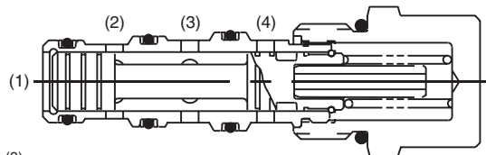
"C" SPOOL — DH103C
